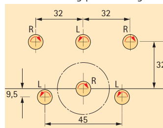
TB 43 Standard drilling pattern hinges
